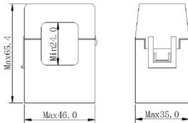
Φ 24mm
